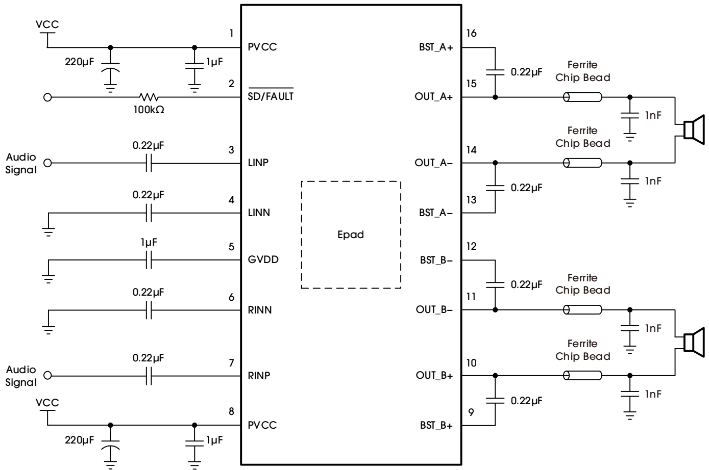
Figure 6. AU3109 BTL Output Reference Schematic
