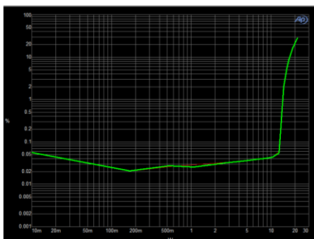
Figure 2. THD+N vs. P_O (BTL, BD Mode, 12V, 6Ω)
