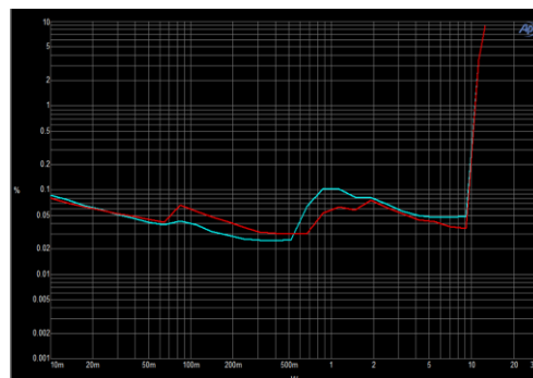
Figure 3. THD+N vs. Frequency (BTL, 1SPW, 12V, 6Ω)
