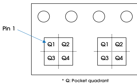
Figure 14. Product Loading Orientation
