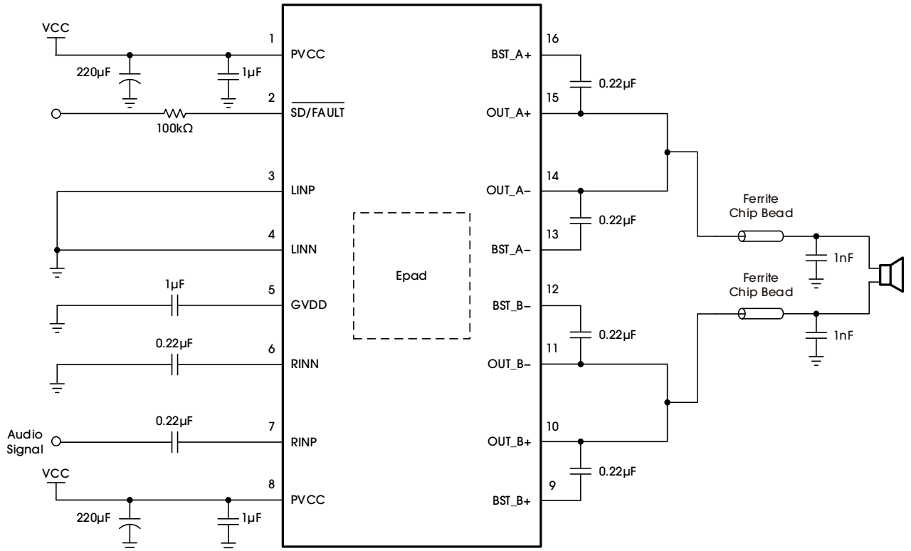
Figure 7. AU3109 PBTl Output Reference Schematic
